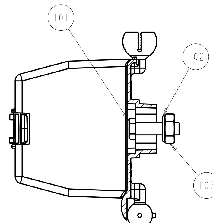
OPTION 2 (IF ATTACHING TO BRACKET WITH CLEARANCE HOLE)
