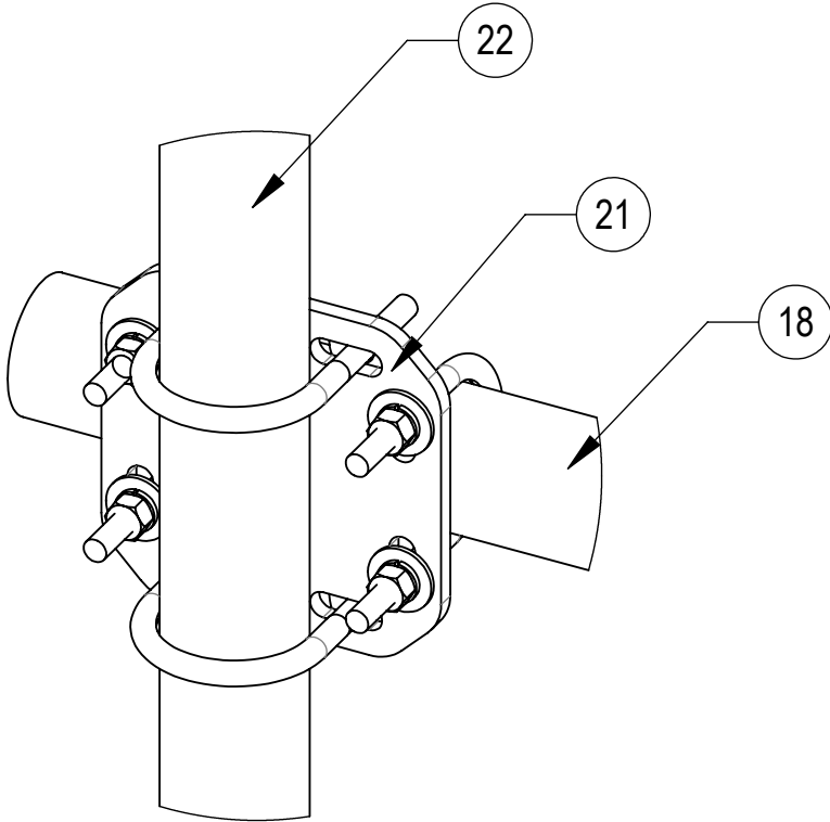
DETAIL G SCALE 1 : 4
