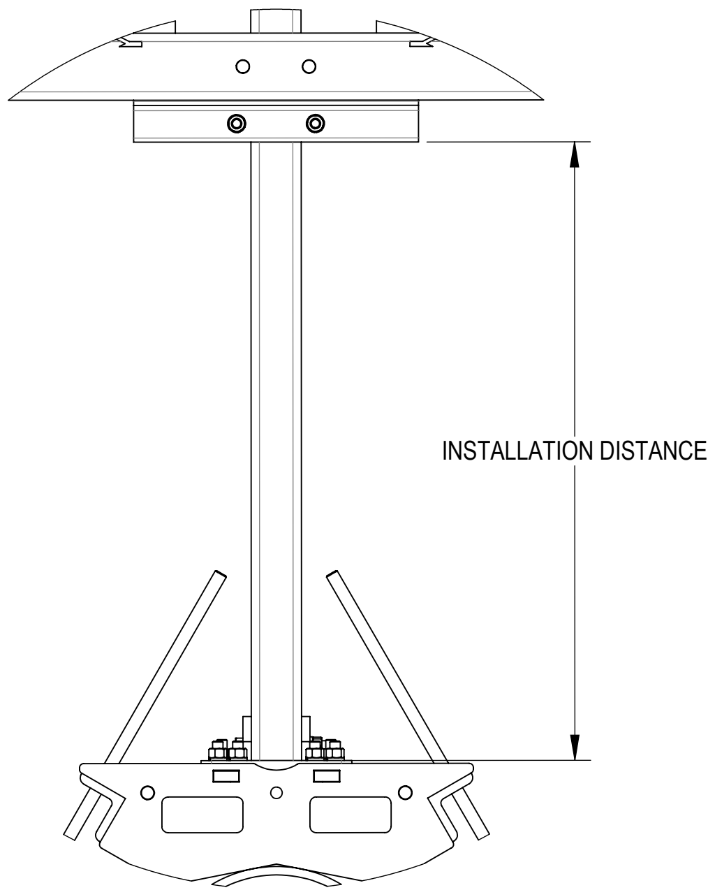
DETAIL X SCALE 1 : 8
