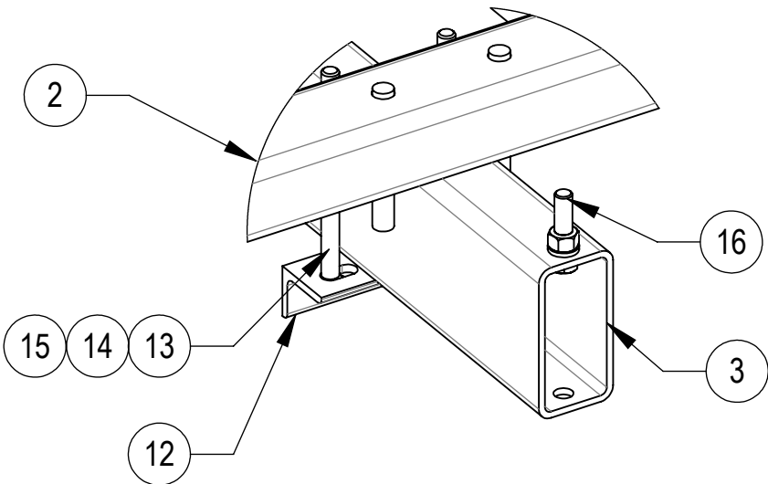
DETAIL C SCALE 1 : 6
