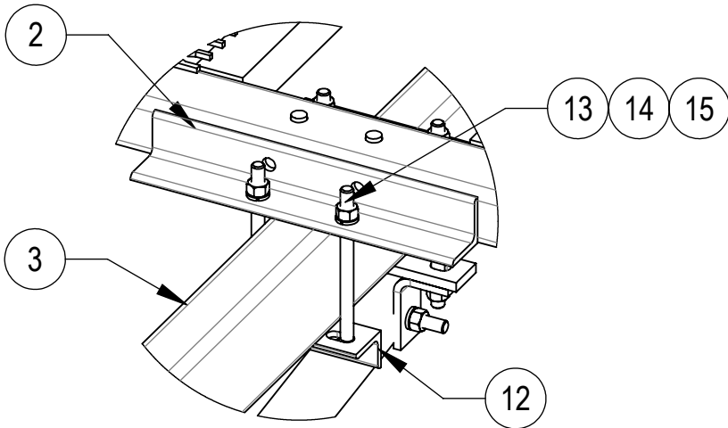
DETAIL B SCALE 1 : 8
