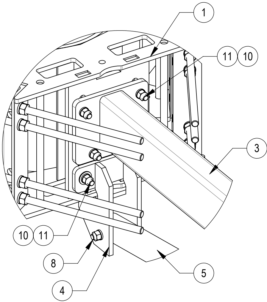
DETAIL A SCALE 1 : 6
