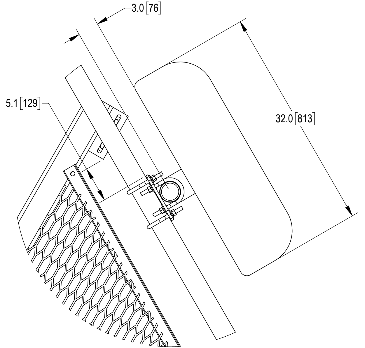
DETAIL V SCALE 1 : 8
