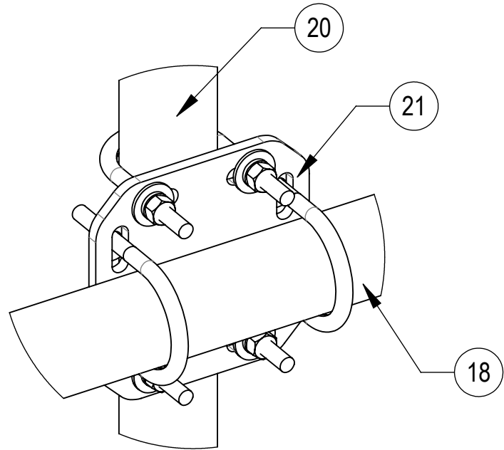
DETAIL T SCALE 1 : 4
