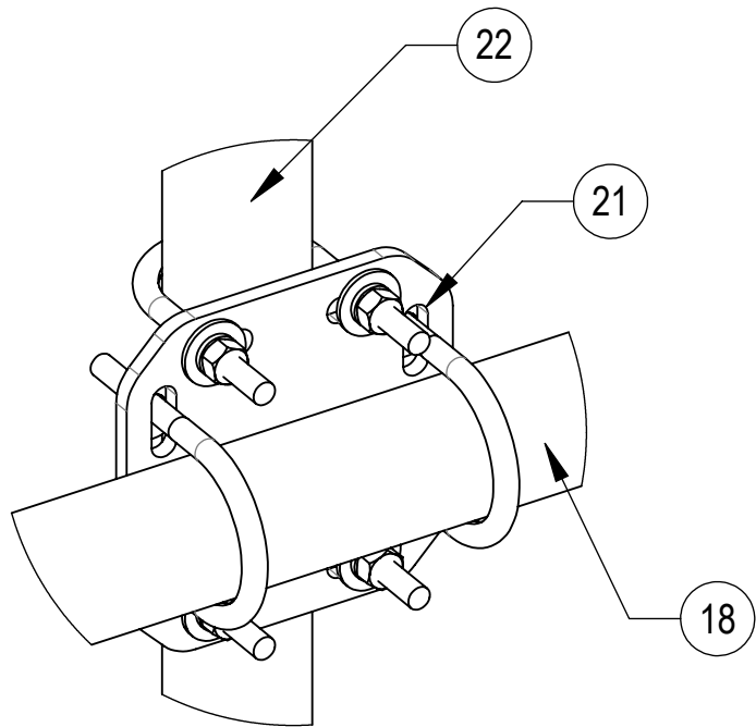
DETAIL W SCALE 1 : 4
