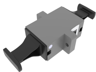
Fiber Optic Adapter, MPO 12, with flanges, with metal clip, aligned key, gray
