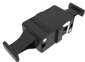
Fiber Optic Adapter, MPO 16, without flanges, with metal clip, opposed key, black
