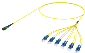
MPO Fanout Cable, polarity A, 12 fiber MPO (unpinned) to LC duplex, Plenum 3mm SM, 7m, with 36" breakout
