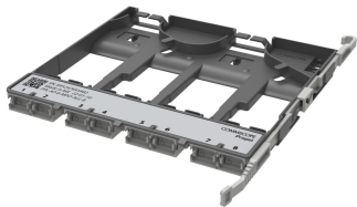
Propel pass-through adapter pack, 8 MPO8-12-24 ports, Type A
