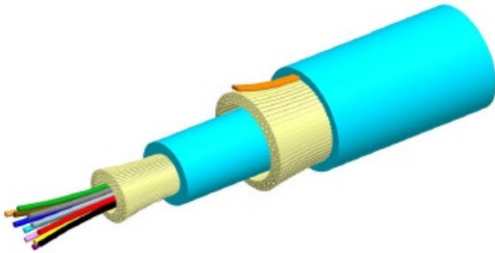
Plenum Light Duty Interconnect cable
